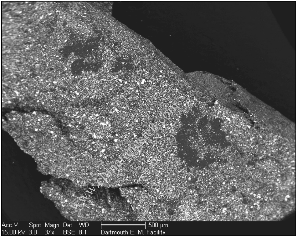
Figure D-1. SEM micrograph of broken surface of tungsten/nylon round.
